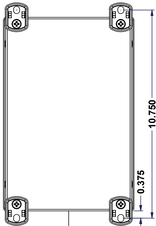
BACK
