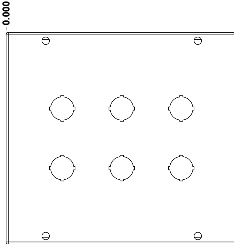
FRONT
