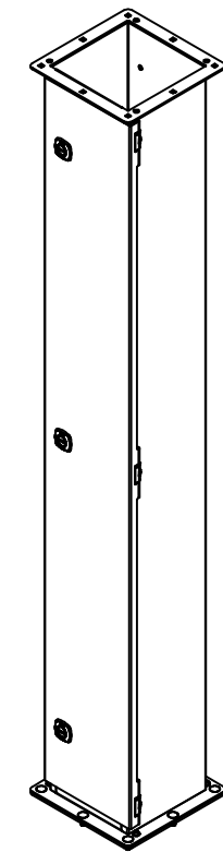
Isometric View
