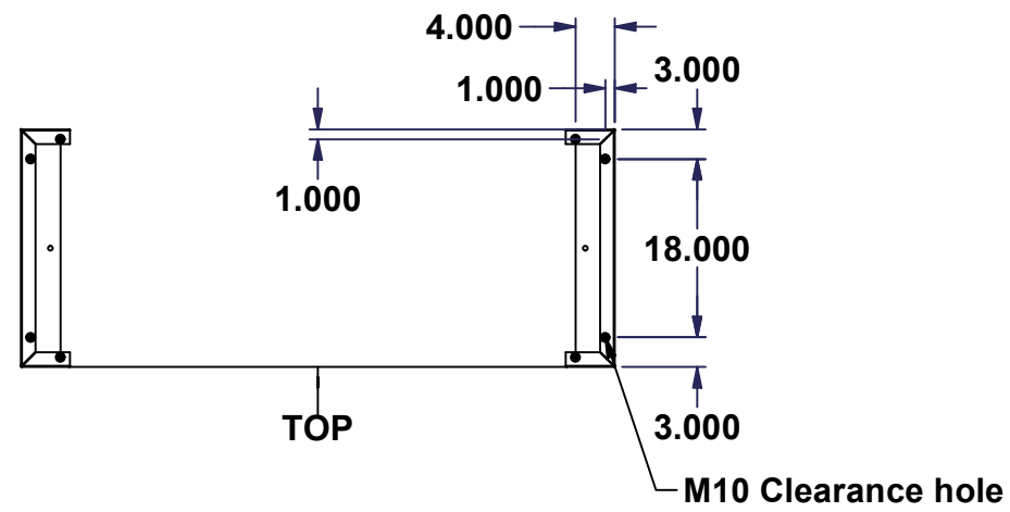
ENCLOSURE CUTOUT LAYOUT
