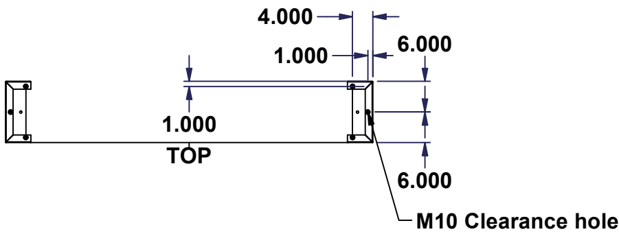
ENCLOSURE CUTOUT LAYOUT
