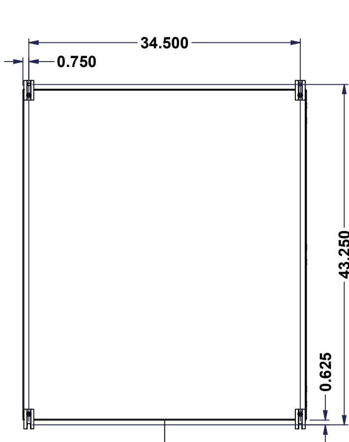
BACK
