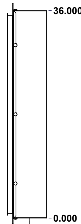
RIGHT
