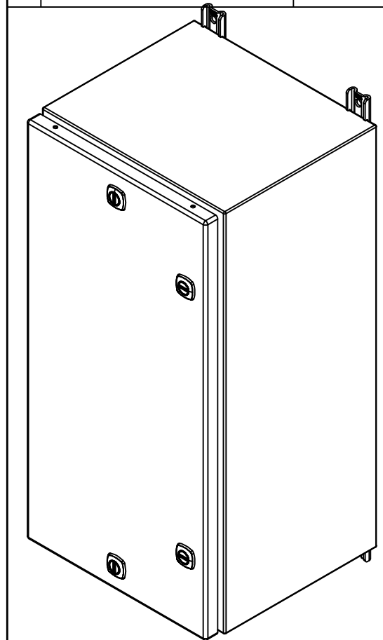
Isometric View
