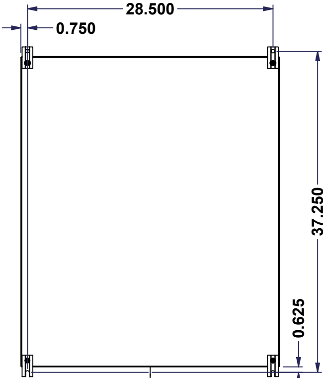
BACK
